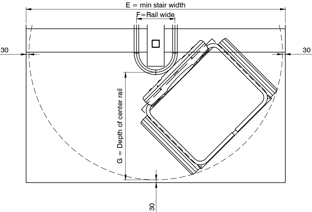
Note Drawing shown as columns mounted rail.
