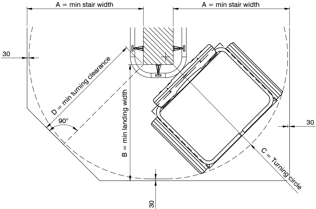
Note Drawing shown as wall mounted rail Can also be columns mounted.
